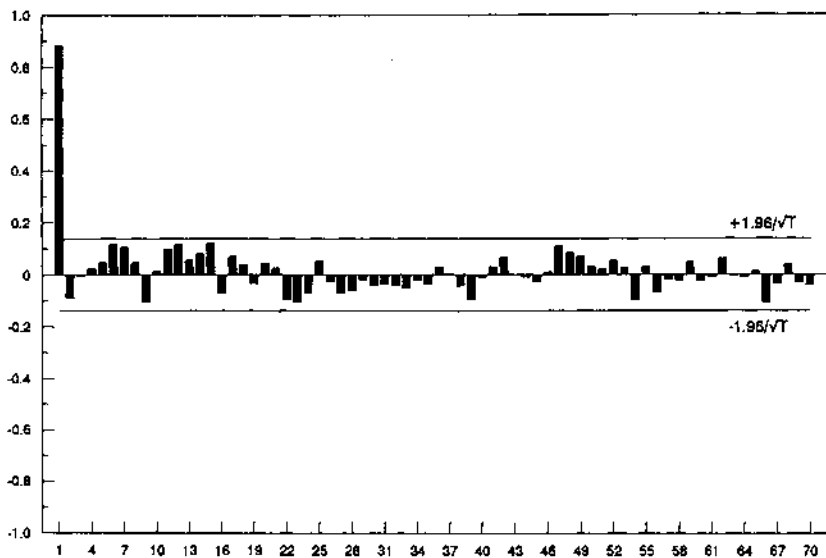
FIG. 3.—Sample partial autocorrelation function for dollar-sterling real exchange rate.
