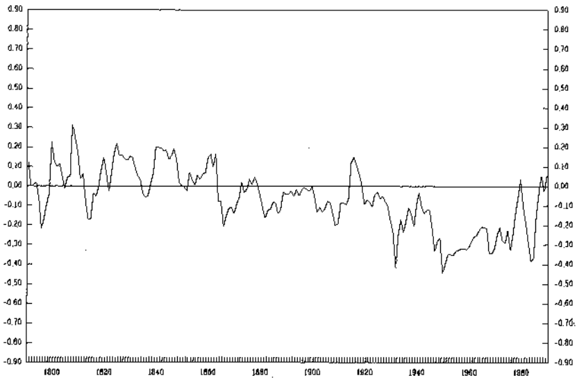
FIG. 1.—Logarithm of dollar-sterling real exchange rate, 1791–1990 (1900 = 0; increase = sterling appreciation).
