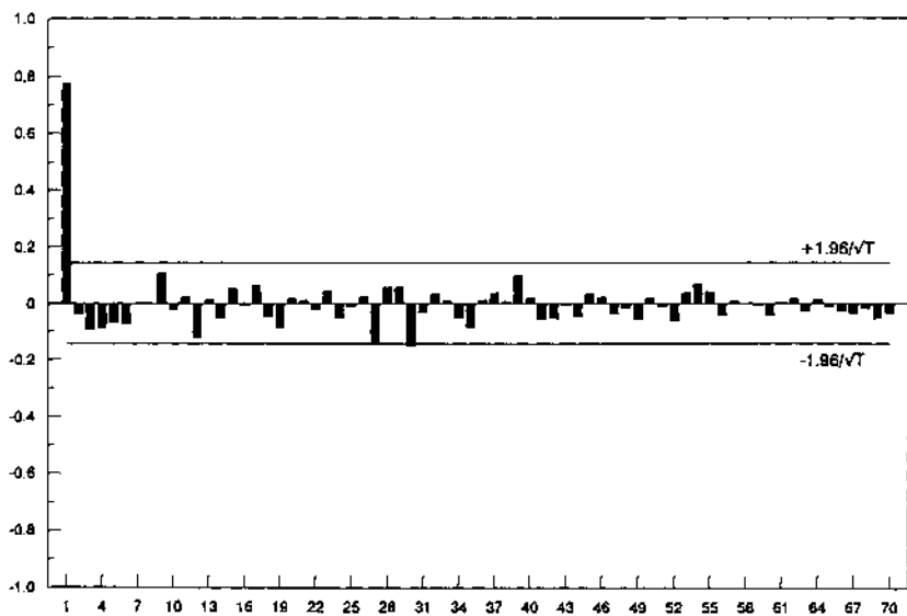
FIG. 5.—Sample partial autocorrelation function for franc-sterling real exchange rate.
