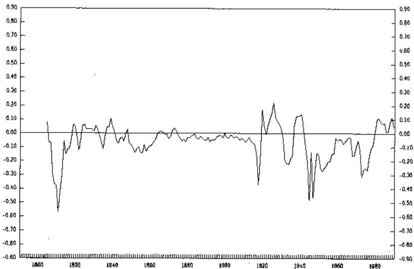
FIG. 2.—Logarithm of franc-sterling real exchange rate, 1805–1990 (1900 = 0; increase = sterling appreciation).
